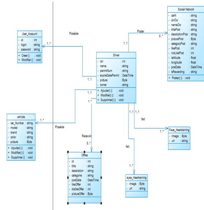
Figure 11. Class diagram for the management of vehicle
