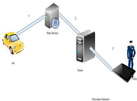
Figure 9. Application architecture
