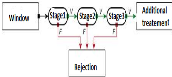
Figure 2. Boosting method
