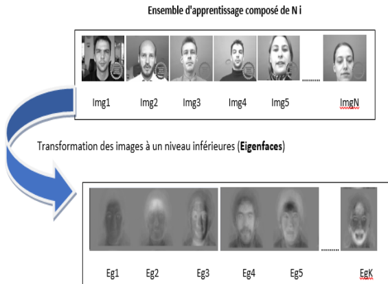
Figure 5. Image Classification
