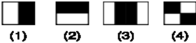
Figure 1. HaarTraining Rectangles
