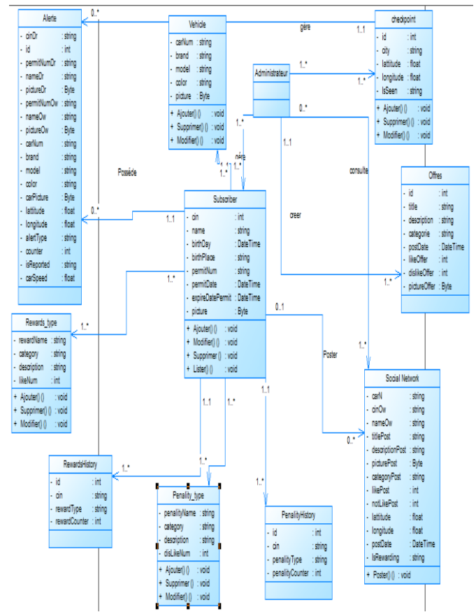
Figure 12. Class diagram for the management of agency
